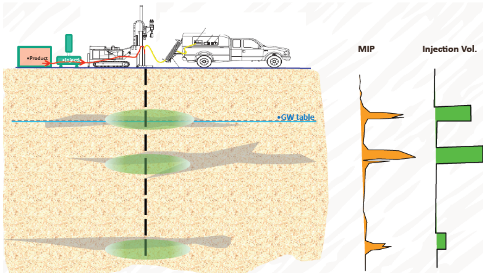
Principle of targeted injection (Grey shadows indicates contamination)
